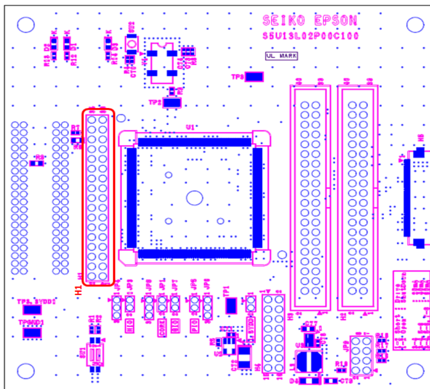
Figure 4-2: Host Bus Connector Location (H1)
