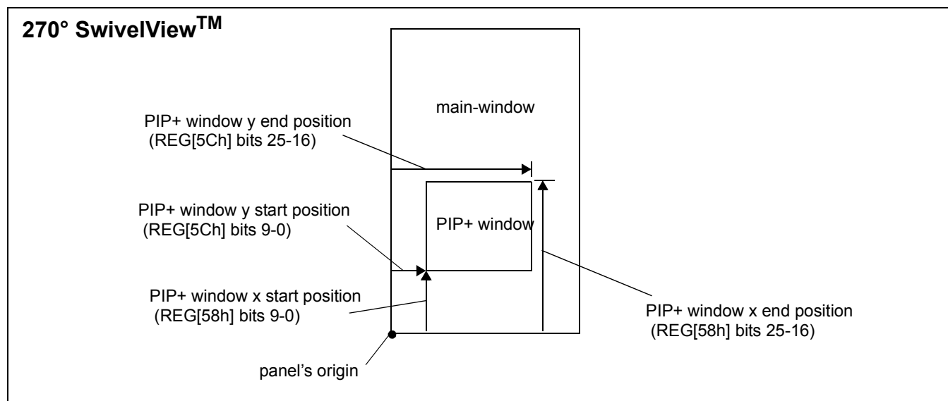
Figure 8-5: Picture-in-Picture Plus with SwivelView 270° enabled
