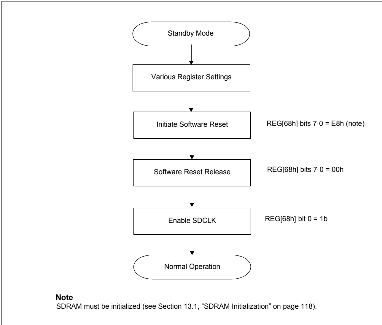
Figure 16-4: Recommended Procedure for Exiting Standby Mode
