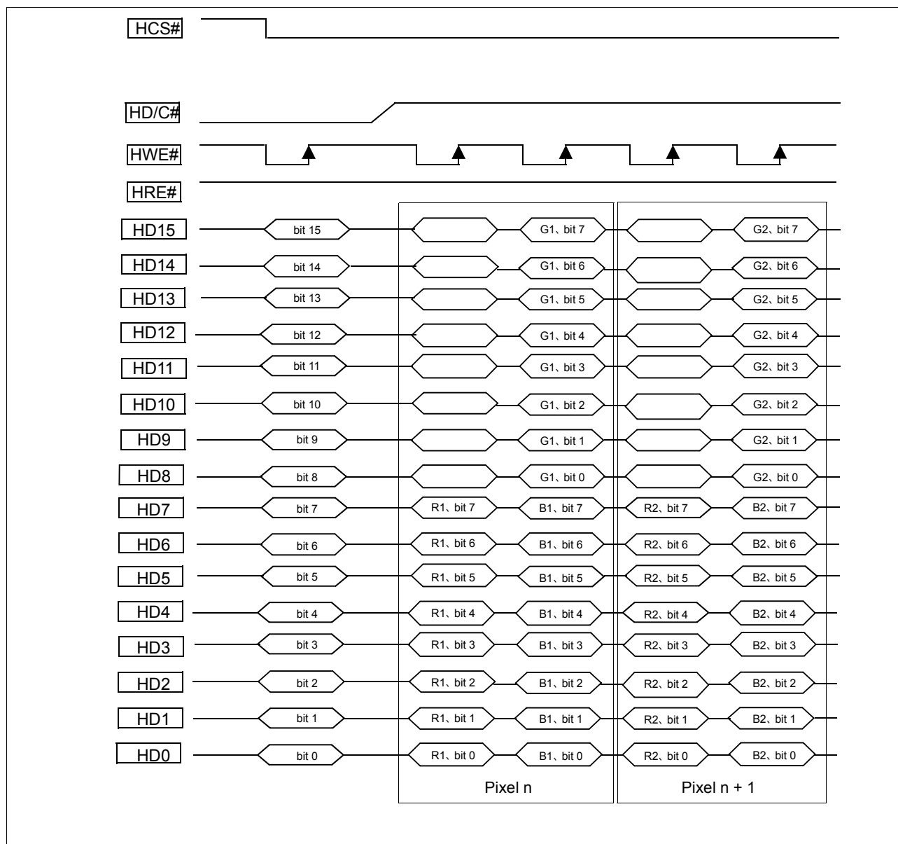
Figure 11-9: 16-bit 24bpp mode 2 (RGB 8:8:8)
