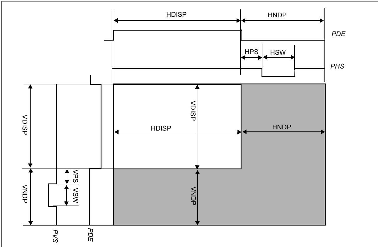
Figure 8-15: Panel Timing Parameters
