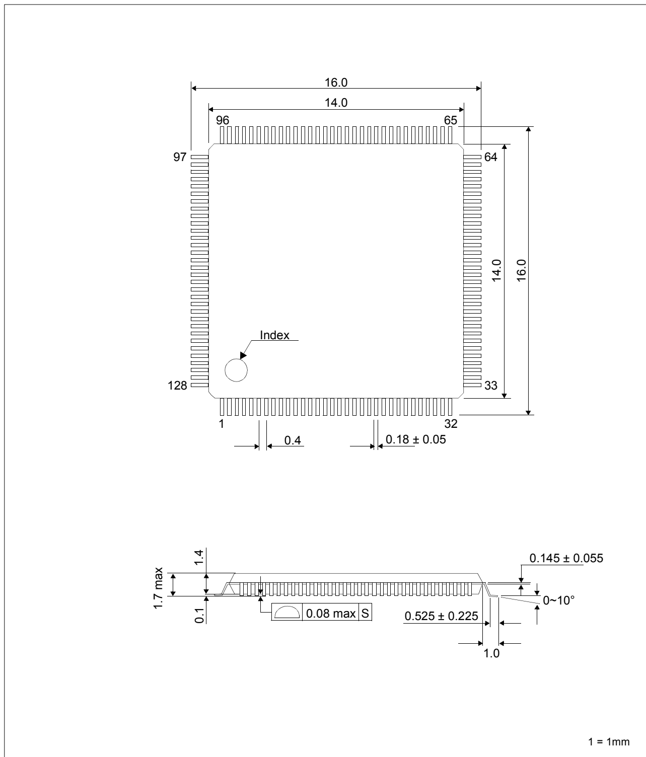
Figure 19-1: QFP15 128-pin Package
