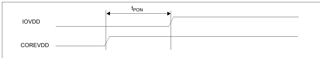
Figure 8-4: Power-on Sequence Timing
