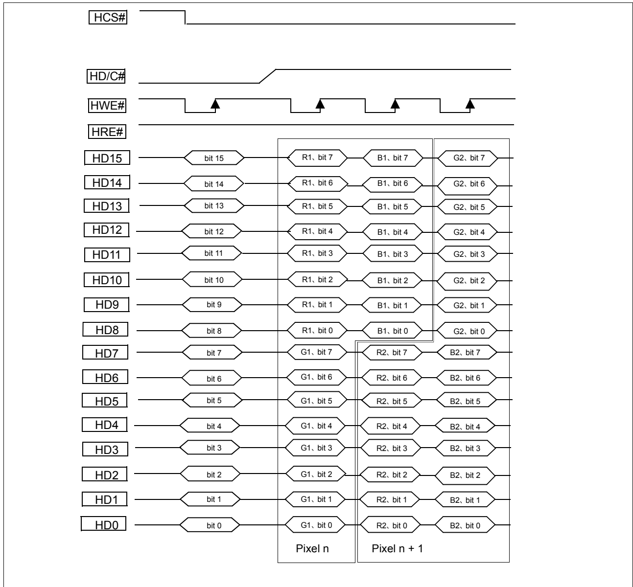
Figure 11-8: 16-bit 24bpp mode 1 (RGB 8:8:8)
