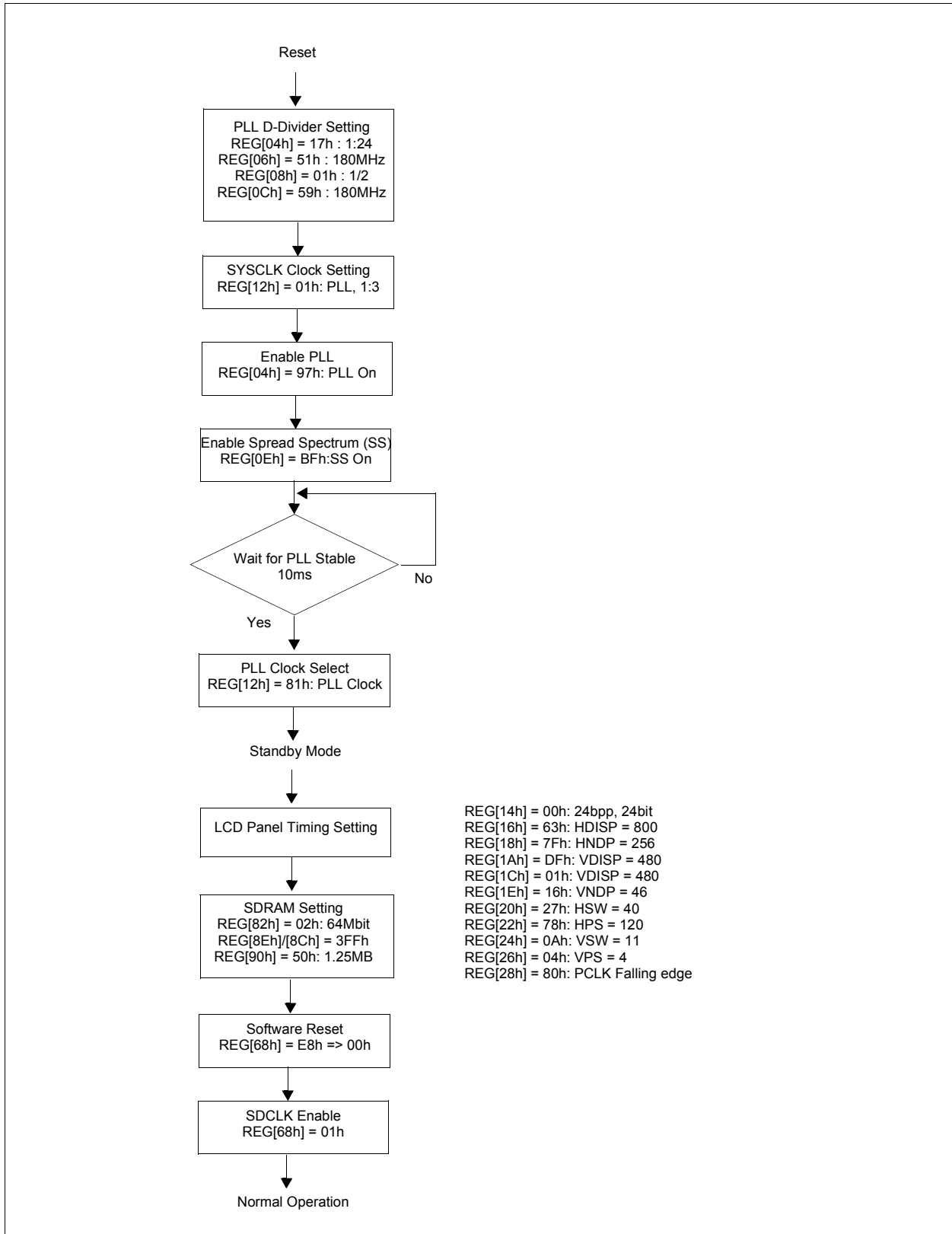
Figure 17-1: Typical S1D13517 Initialization Sequence
