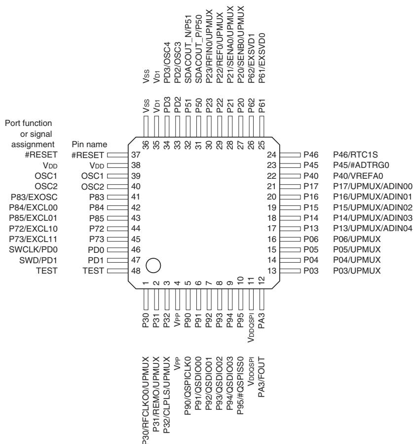
Figure 1.3.1.1 S1C31D50/D51 Pin Configuration Diagram (TQFP12-48PIN)
