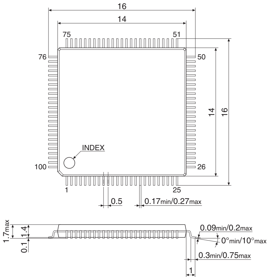
Figure 24.4 QFP15-100PIN Package Dimensions
