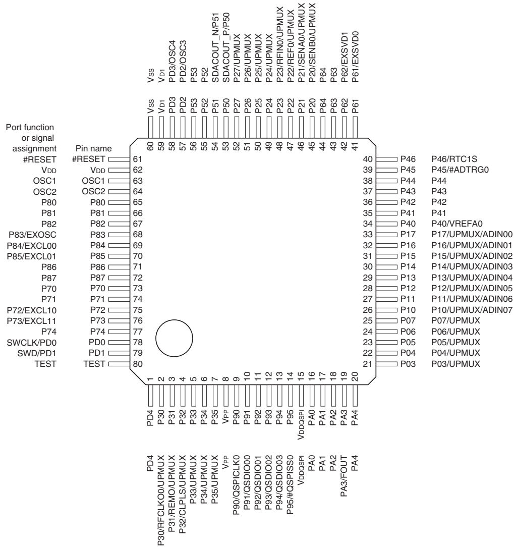
Figure 1.3.1.3 S1C31D50/D51 Pin Configuration Diagram (QFP14-80PIN)
