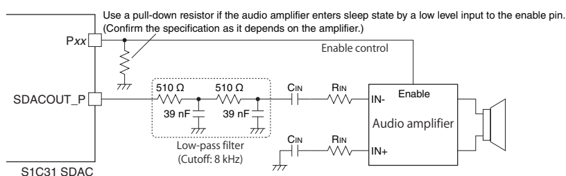
Figure 21.2.2.1 Single Mode Connection Example
