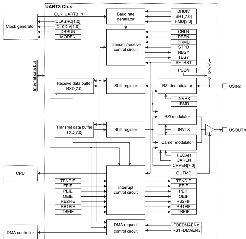
Figure 13.1.1 UART3 Configuration
