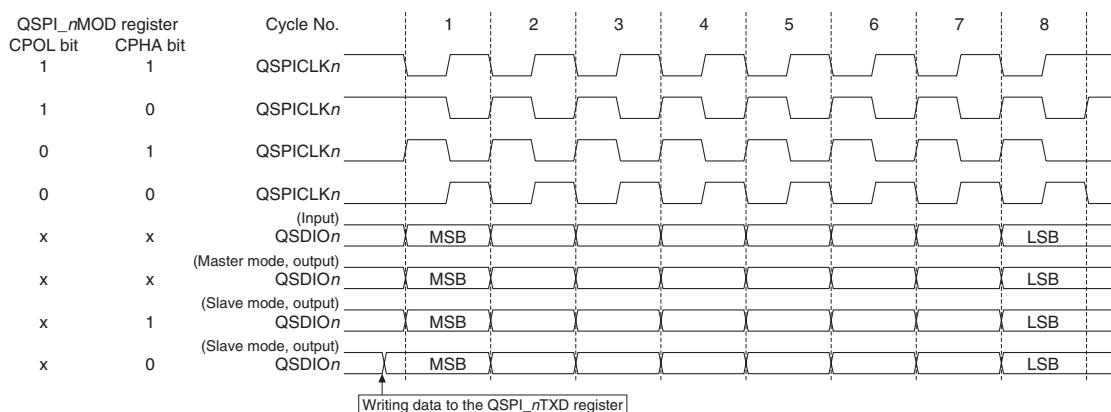
Figure 15.3.3.1 QSPI Clock Phase and Polarity (QSPI_nMOD.LSBFST bit = 0, QSPI_nMOD.CHLN[3:0] bits = 0x7)
