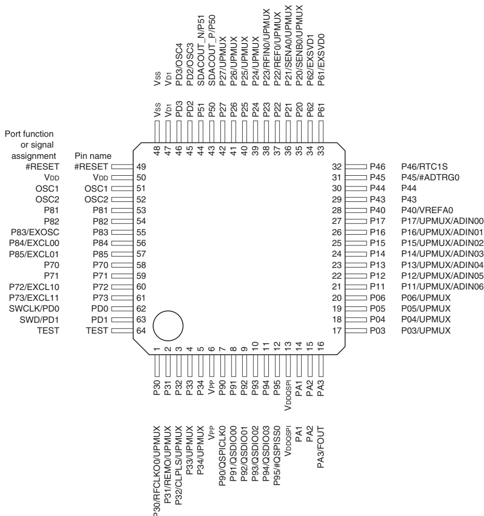
Figure 1.3.1.2 S1C31D50/D51 Pin Configuration Diagram (QFP13-64PIN)
