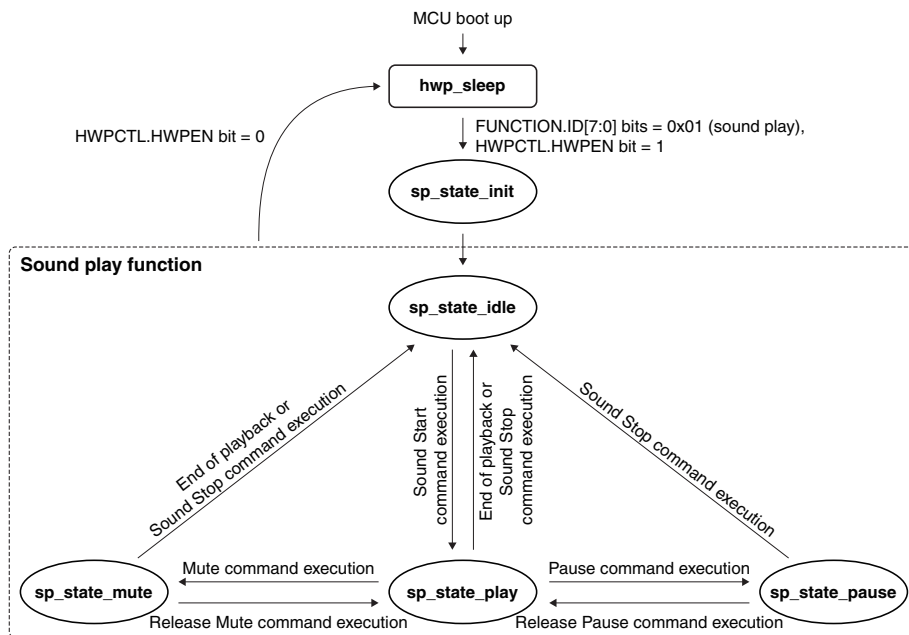
Figure 21.4.1.1 Sound Play State Transition Diagram
