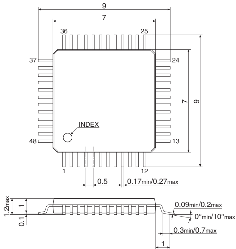
Figure 24.1 TQFP12-48PIN Package Dimensions
