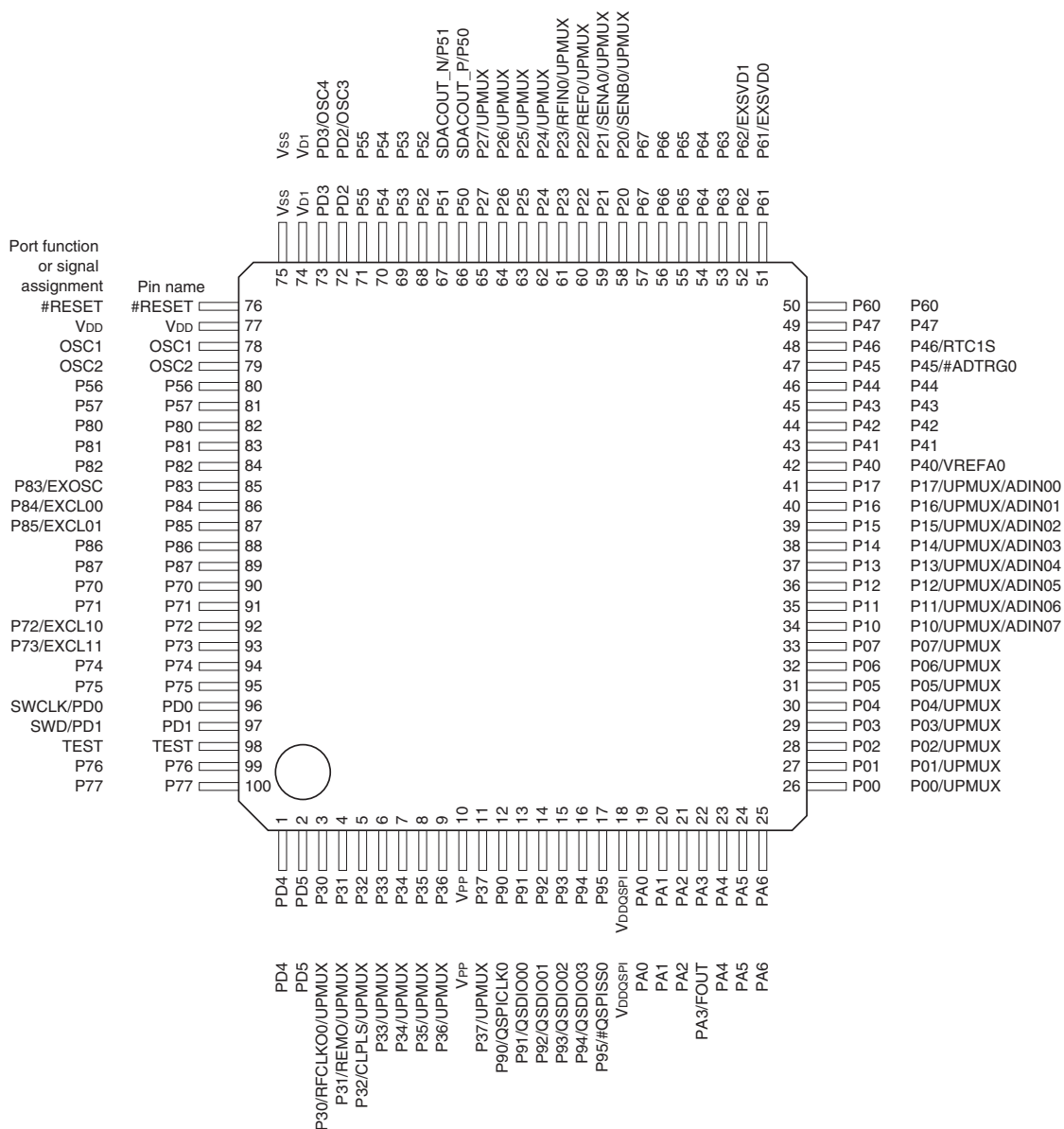
Figure 1.3.1.4 S1C31D50/D51 Pin Configuration Diagram (QFP15-100PIN)
