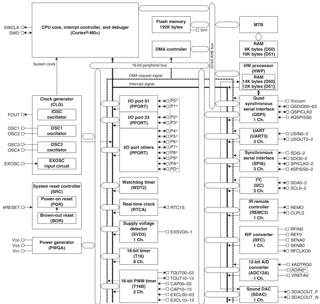
Figure 1.2.1 S1C31D50/D51 Block Diagram
