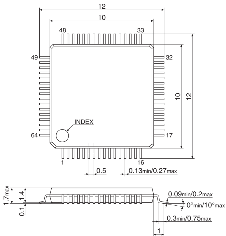
Figure 24.2 QFP13-64PIN Package Dimensions
