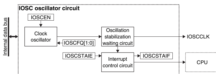
Figure 2.3.3.1 IOSC Oscillator Circuit Configuration
