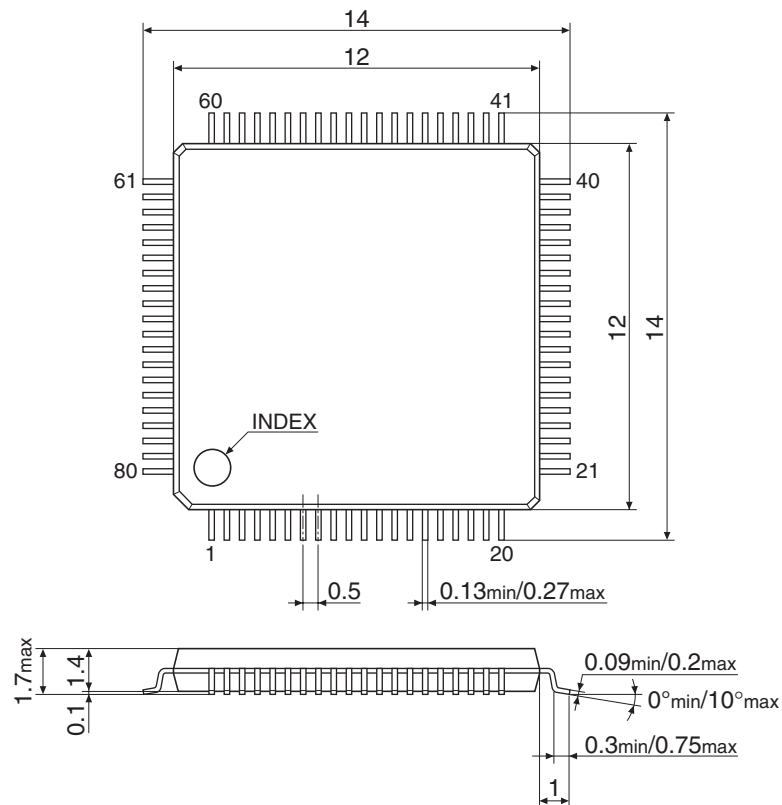
Figure 24.3 QFP14-80PIN Package Dimensions
