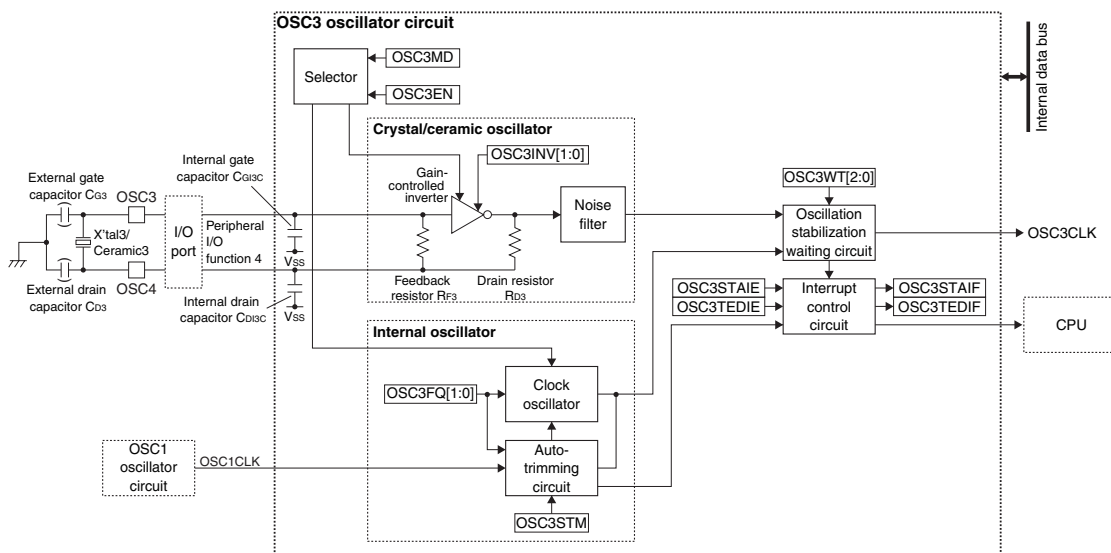
Figure 2.3.3.3 OSC3 Oscillator Circuit Configuration
