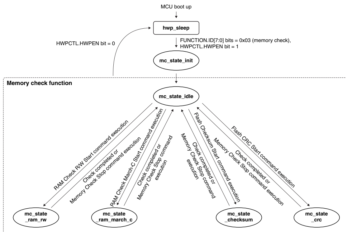
Figure 21.4.2.1 Memory check State Transition Diagram
