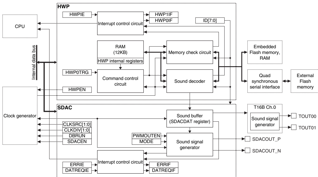
Figure 21.1.1 HWP Configuration
