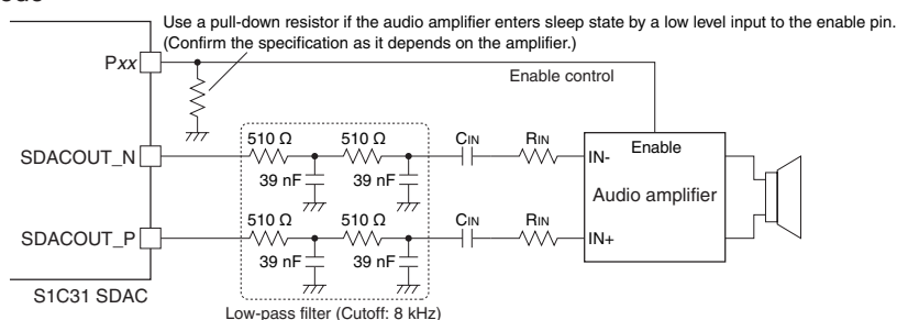
Figure 21.2.2.2 Differential Mode Connection Example
