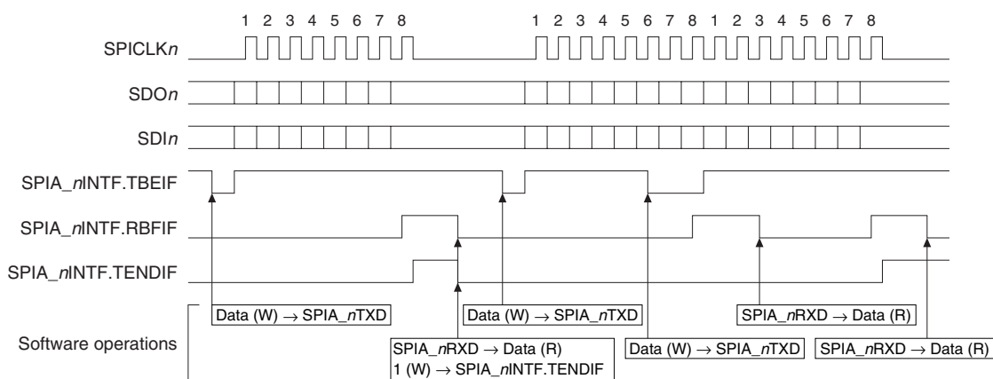
Figure 14.5.3.1 Example of Data Receiving Operations in Master Mode (SPIA_nMOD.CHNLN[3:0] bits = 0x7)
