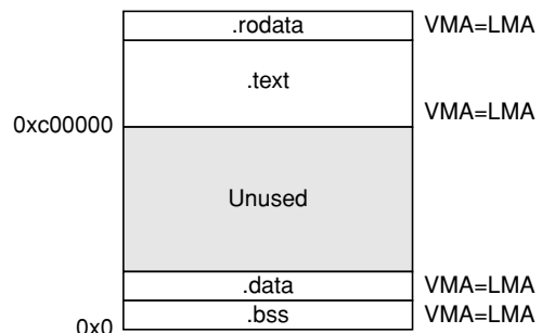
Figure 9.4.2.1 Memory map configured by default script
