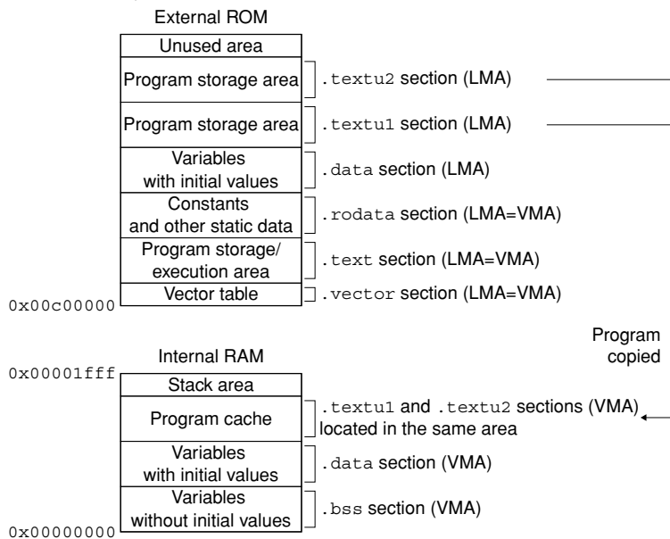
Figure 5.7.7.8 Allocating a storage area for the program in RAM
