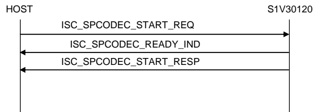
Figure 27 Speech Codec START Message Flow (INDICATION before RESPONSE)
