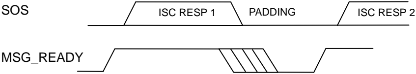
Figure 4 MSG_READY timing
