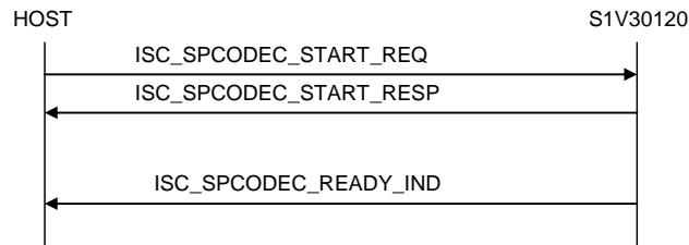
Figure 26 Speech Codec START Message Flow (RESPONSE before INDICATION)
