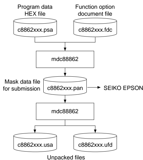
Fig. 3.3.2.1 mdc88862 execution flow
