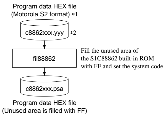
Fig. 3.1.2.1 fil88862 execution flow
