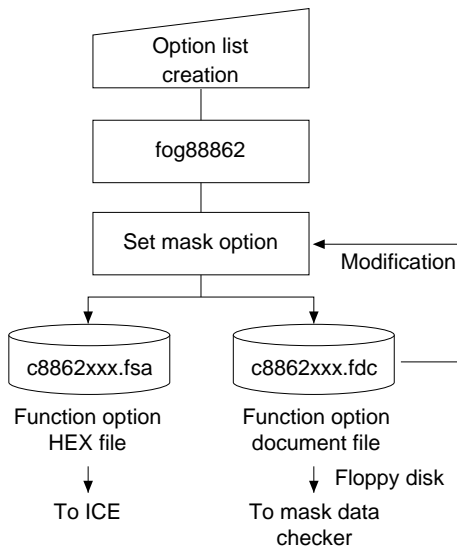
Fig. 3.2.2.1 fog88862 execution flow
