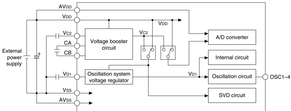
Fig. 2.1.1 Configuration of power supply
