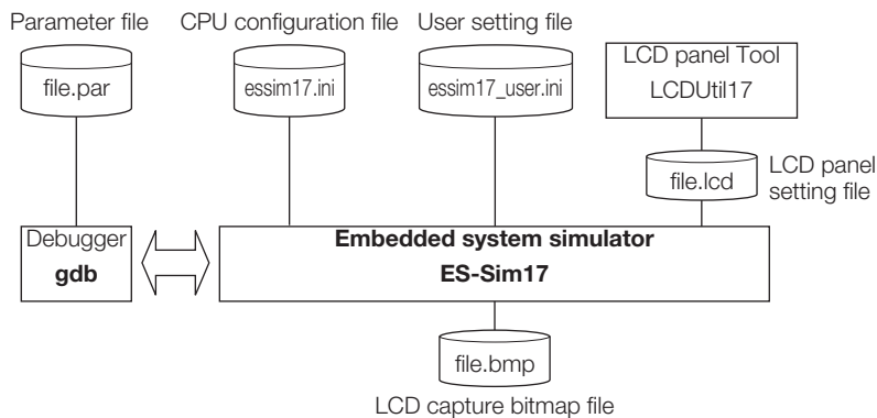
Figure 10.11.1.1 Input/output files
