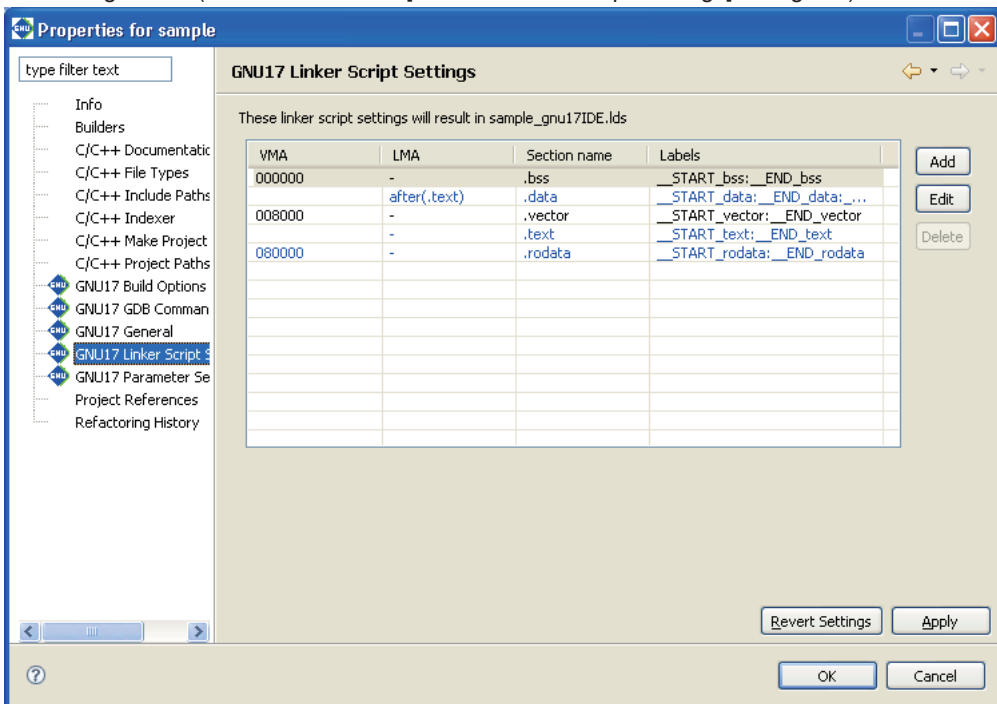
Section configuration (contents set in the [GNU17 Linker Script Settings] dialog box)
