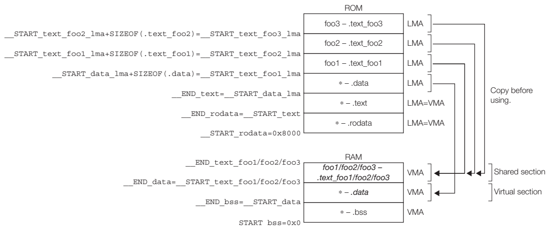
Figure 9.4.2.1 Memory map
