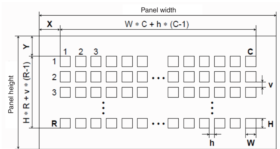
Figure 11.11.6.1.1 Dot matrix setting
