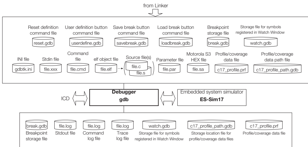
Figure 10.2.1 Flowchart
