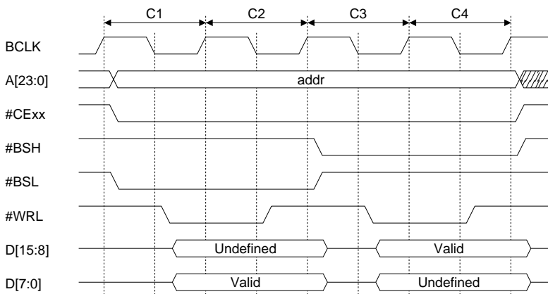
Figure 4.24 Byte Write Cycle with No Wait (#BSL system, little endian)
