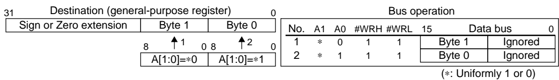
Figure 4.14 Half-word Data Reading from an 8-bit Device
