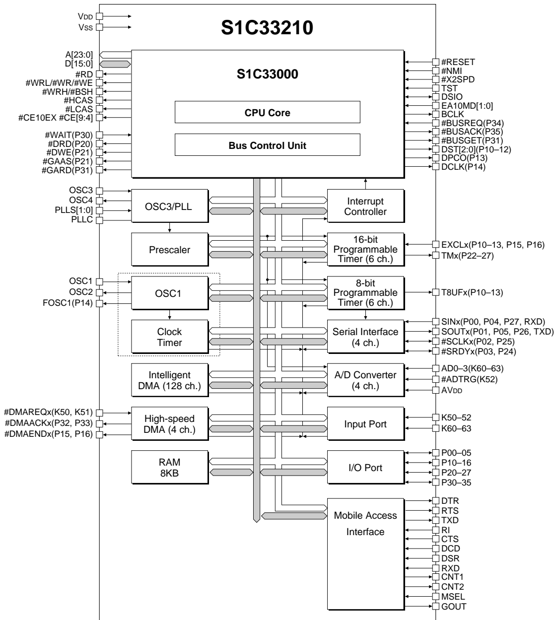
Figure 1.2.1 S1C33210 Block Diagram
