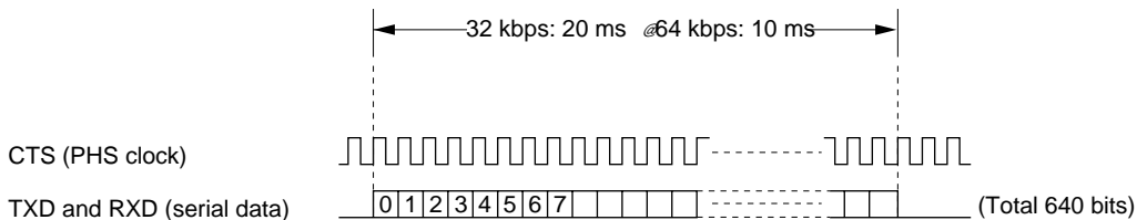
Figure 10.10 PHS Communications Data Format
