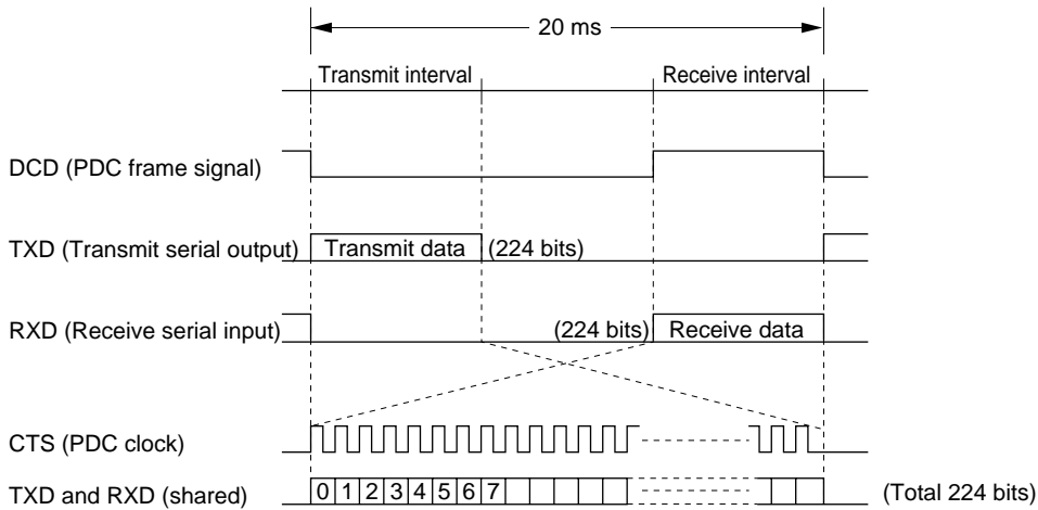
Figure 10.7 PDC Communications Data Format
