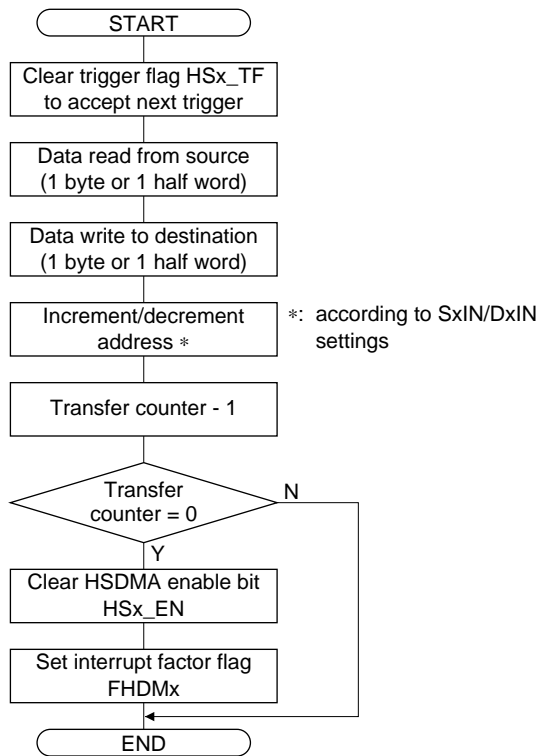
Figure 2.3 Operation Flow in Single Transfer Mode
