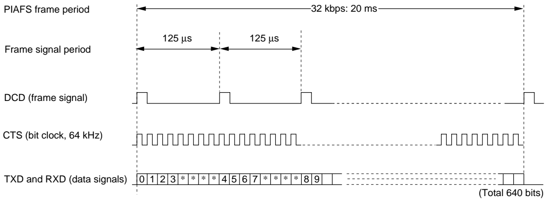
Figure 10.6 PHS Signal Format (5)
