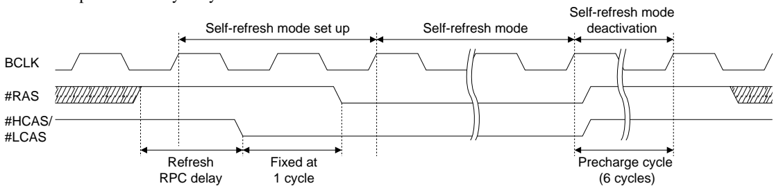
Figure 4.37 Self-Refresh
