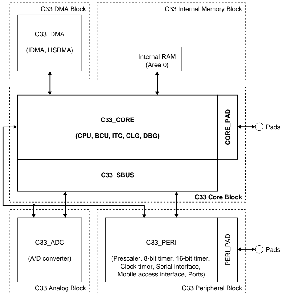
Figure 1.1 Core Block
