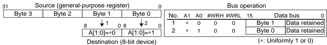
Figure 4.13 Half-word Data Writing to an 8-bit Device
