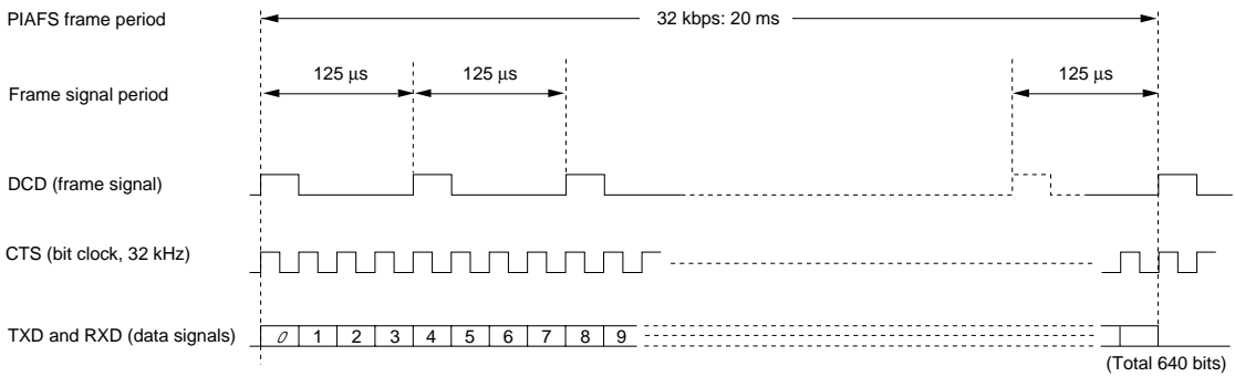
Figure 10.4 PHS Signal Format (3)
