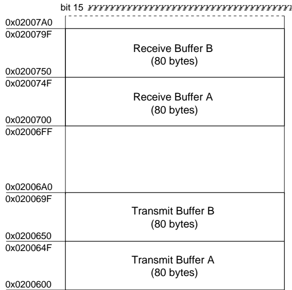
Figure 10.11 PHS Communications Mode Data Buffers
