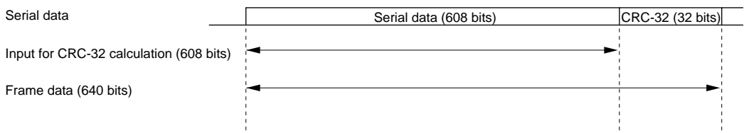
Figure 10.12 PHS Communications Mode FCS (CRC) Position
