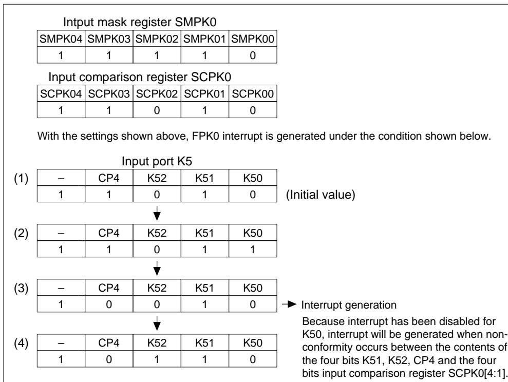
Figure 9.5 FPK0 Interrupt Generation Example (when K5[2:0] and CP4 are selected by SPPK[1:0])
