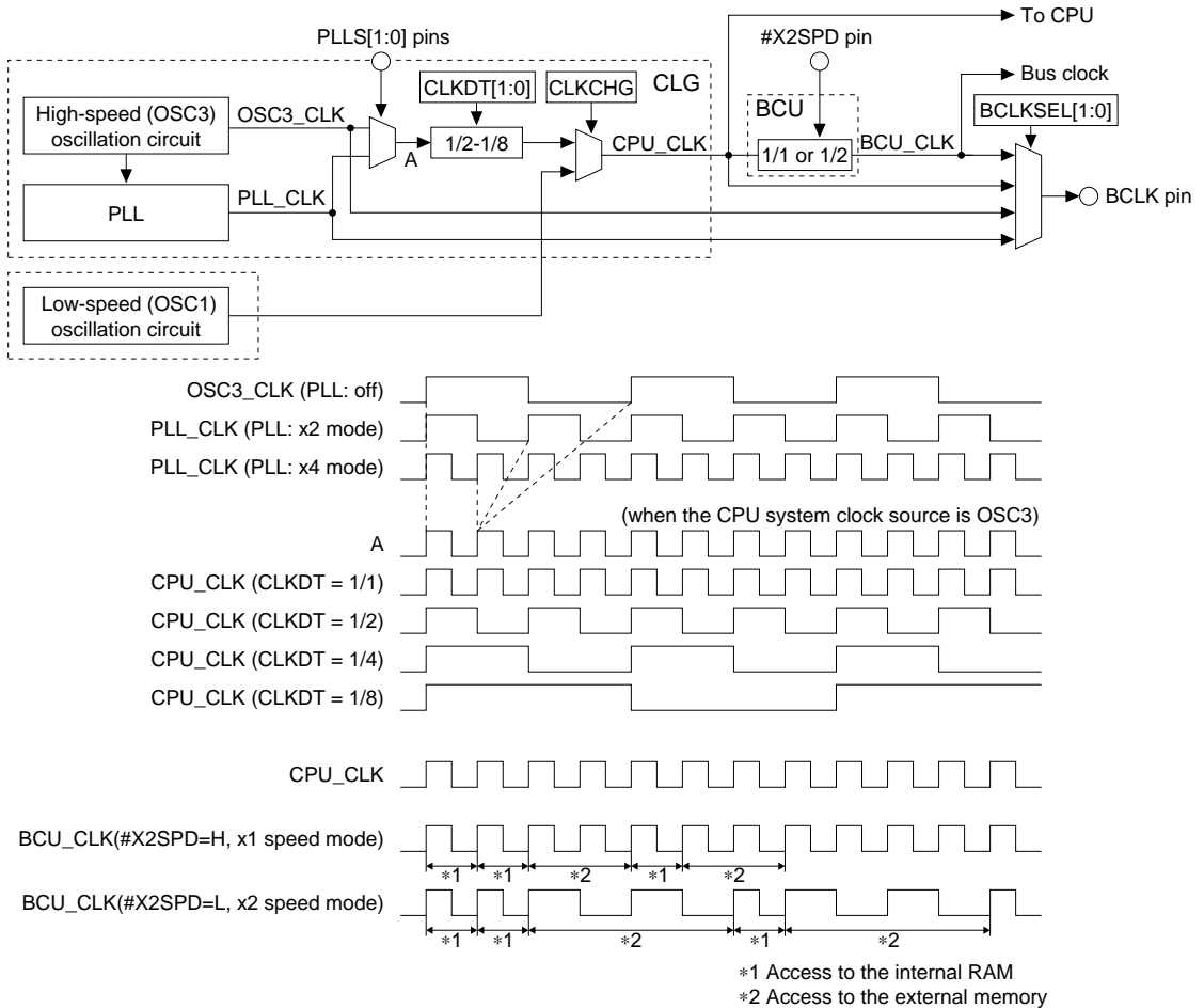
Figure 4.17 Clock System
