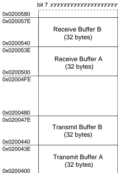
Figure 10.8 PDC Communications Mode Data Buffers
