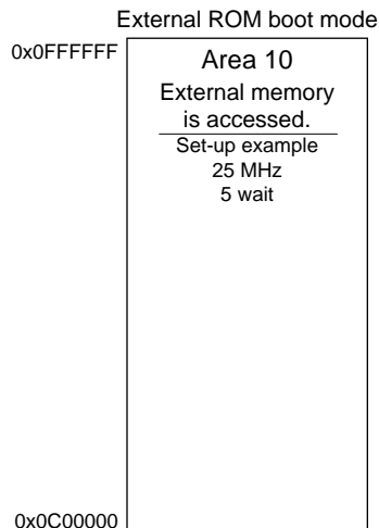
Figure 4.4 Area 10 Memory Map
