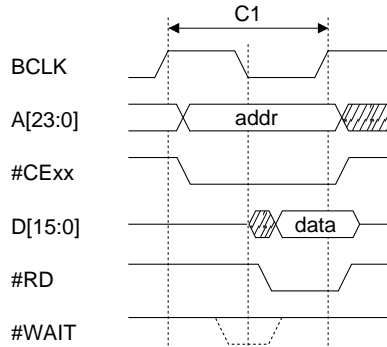
Figure 4.19 Basic Read Cycle with No Wait
