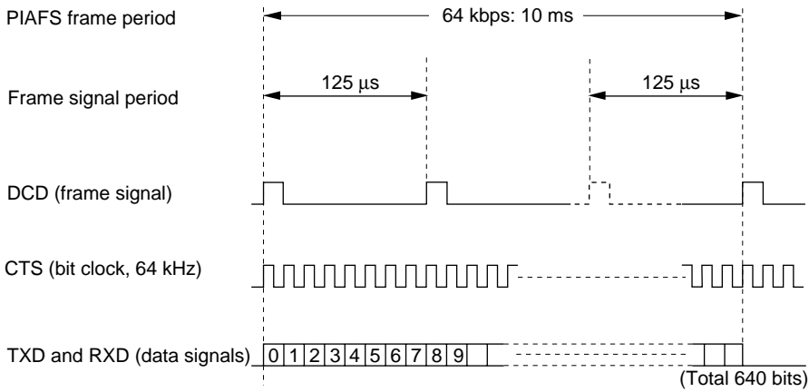
Figure 10.5 PHS Signal Format (4)
