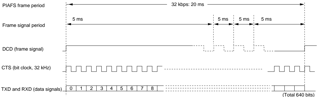
Figure 10.2 PHS Signal Format (1)
