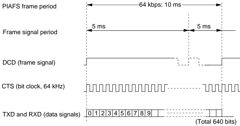
Figure 10.3 PHS Signal Format (2)
