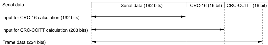
Figure 10.9 PDC Communications Mode
