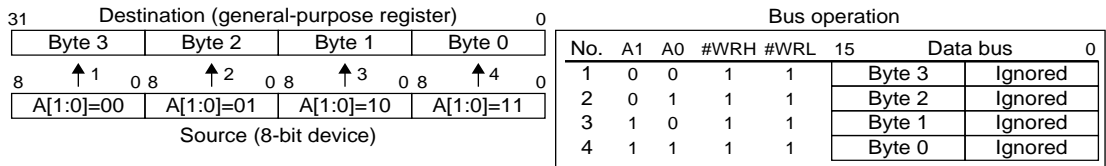
Figure 4.12 Word Data Reading from an 8-bit Device
