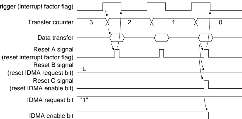
Figure 5.3 Sequence when DINTEN = "0"
