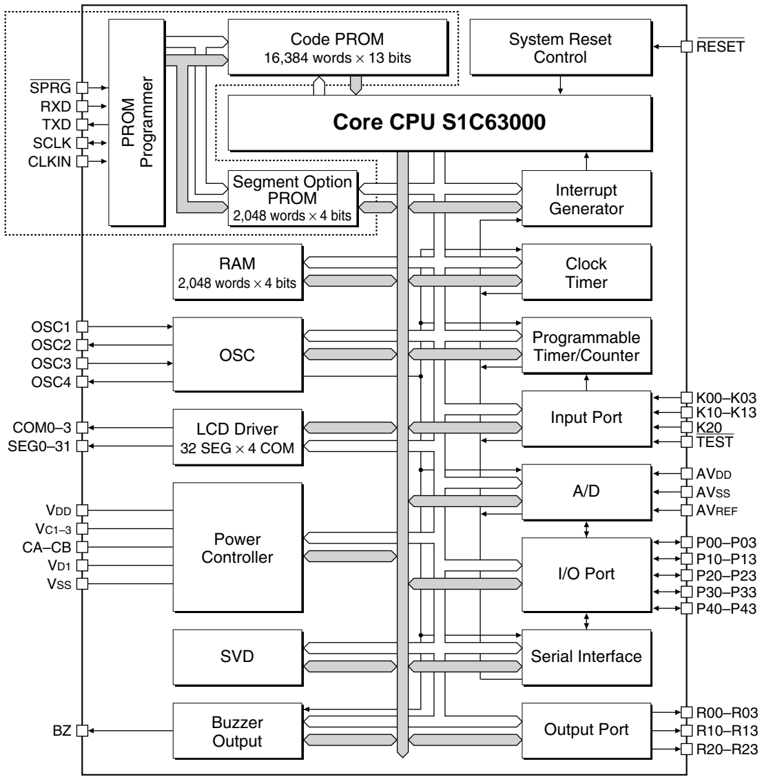
Fig. 1.2.1 Block diagram
