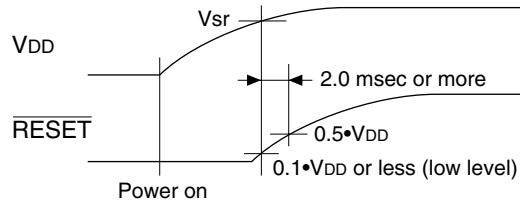
Fig. 6.1.4.1 Initial reset at power-on
