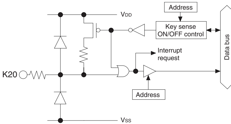
Fig. 4.4.1.2 Configuration of input port (K20)
