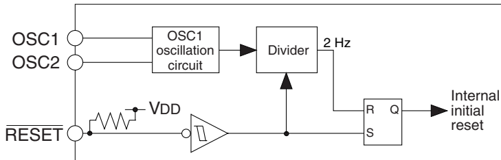
Fig. 2.2.1 Configuration of initial reset circuit
