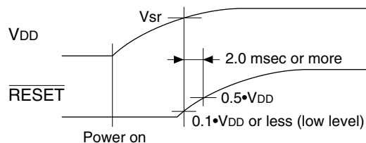
Fig. 6.2.4.1 Initial reset at power-on
