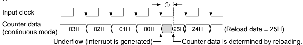
Fig. 7.2.2 Reload timing for programmable timer
