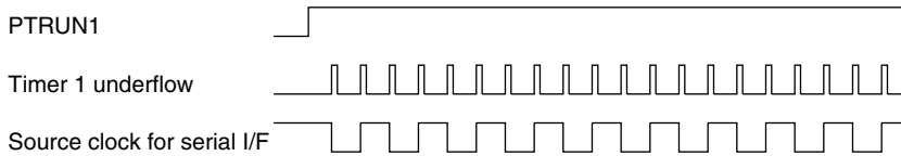
Fig. 4.9.2.6.1 Synchronous clock of serial interface
