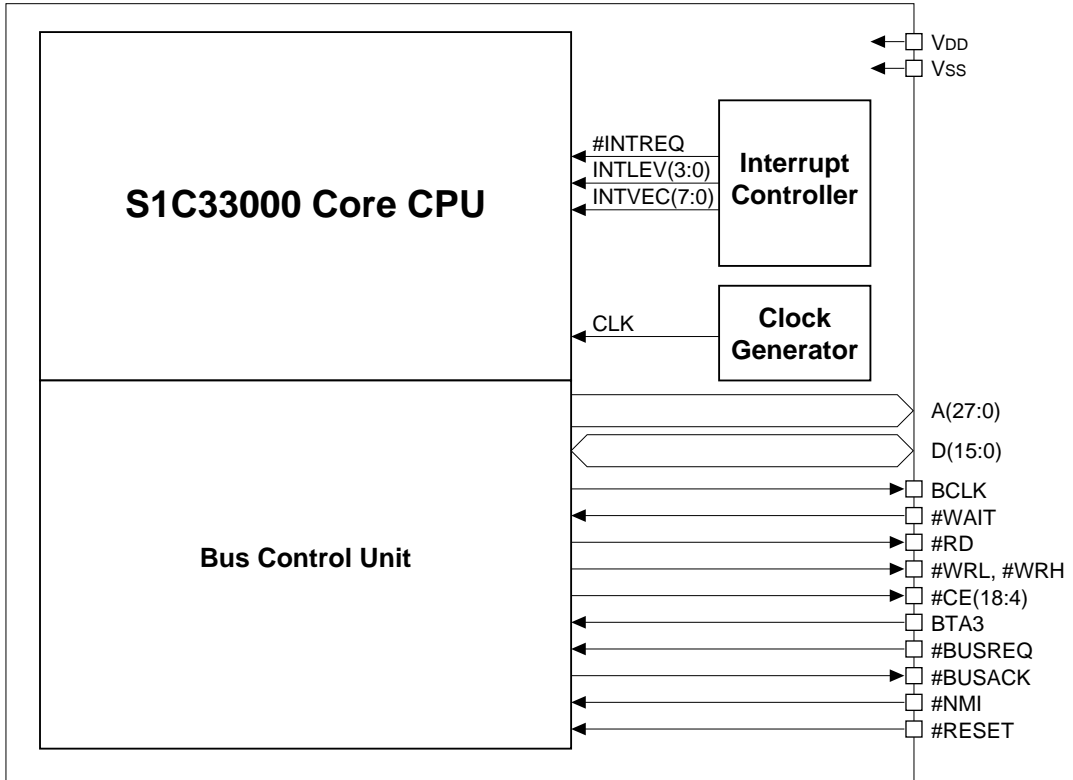
Fig. 1.2.1 S1C33000 block diagram
