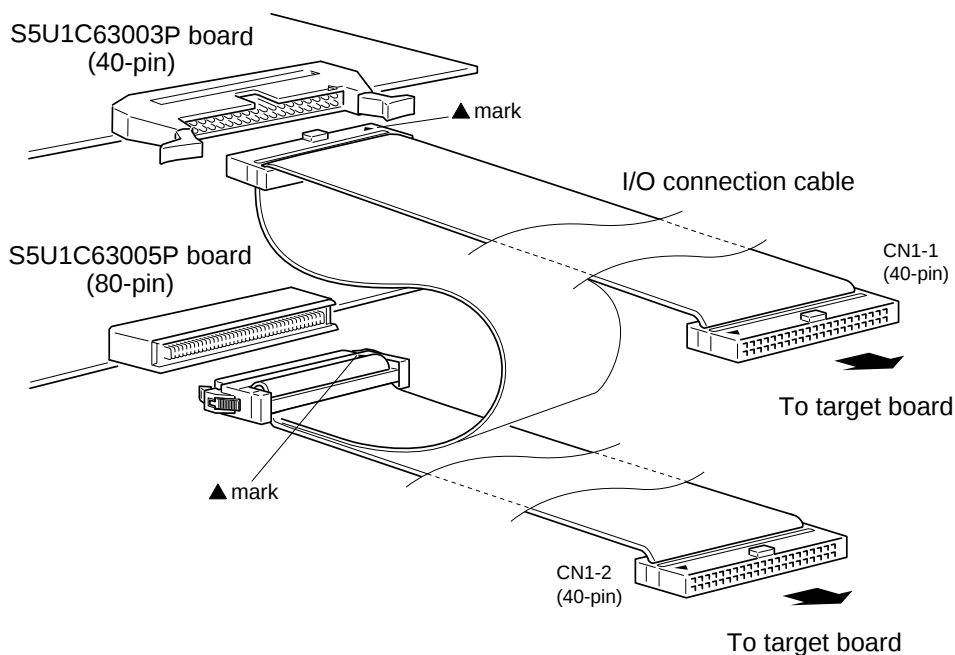
Fig. 5.1 Connecting the S5U1C63005P to the target system
