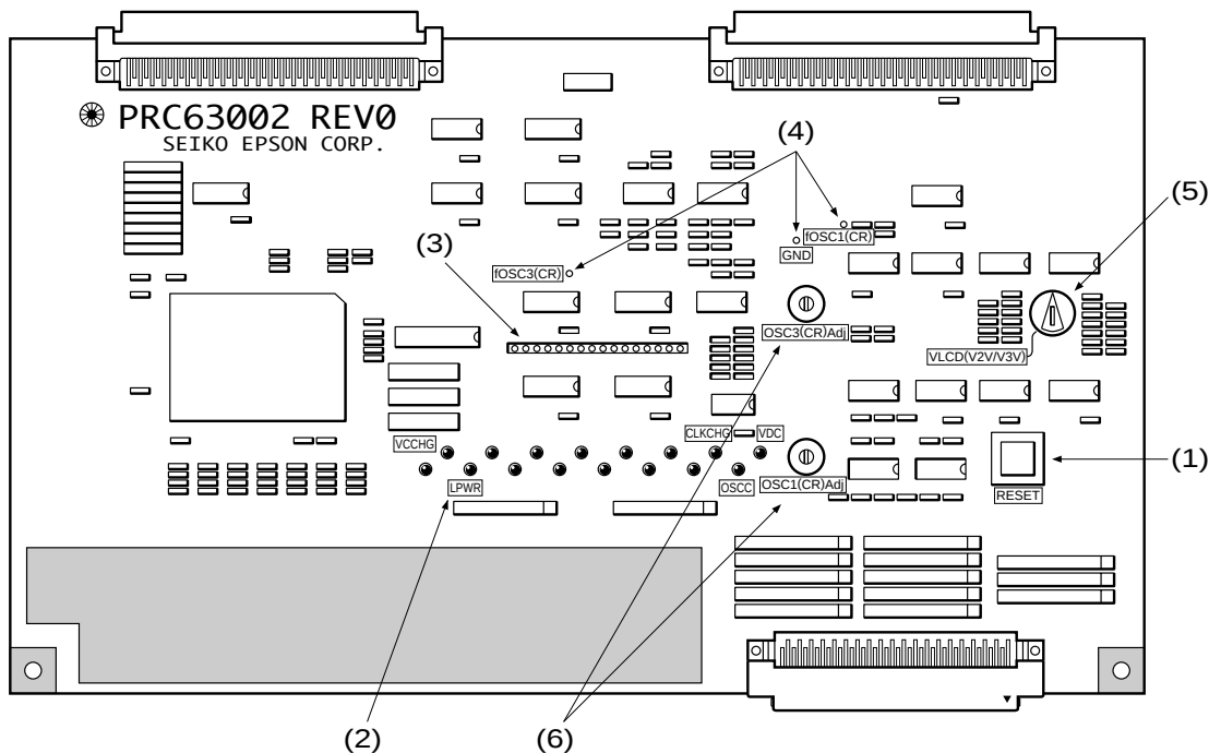
Fig. 4.1 Top view of the S5U1C63005P board
