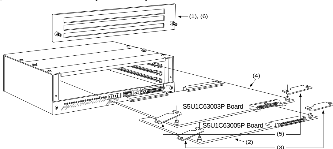
Fig. 2.1.1 Installing the S5U1C63005P board in the ICE
