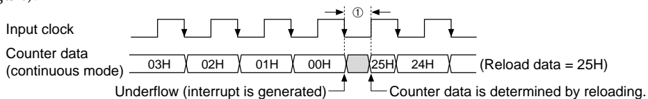
Fig. 4.11.5.2 Reload timing for programmable timer
