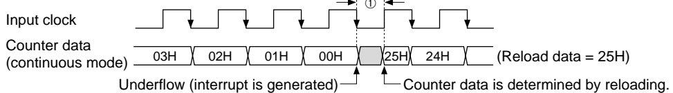
Fig. 5.2.2 Reload timing for programmable timer
